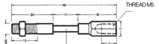
MIS-ALIGNMENT SPRING MAX MIS - ALIGNMENT 3MM
