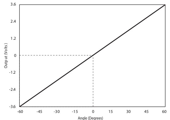
Analog Output
