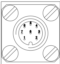
Front view of housing connector inclinometer
