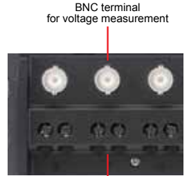
M3 screw terminal for temperature measurement ‡ Connections are made to both the BNC terminal and M3 screw terminal for the same channel.
