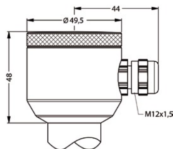
compact field housing (IP 67) ventilation tube
